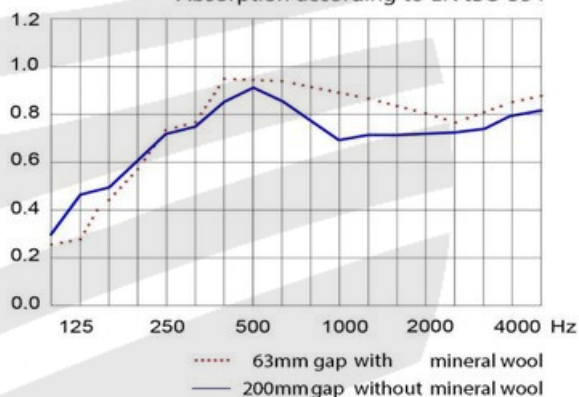
Absorption according to EN ISO 354
